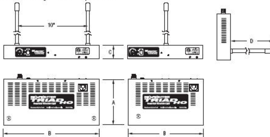
Fig. 3 Dimensions of single and dual lamp Triad HO.
